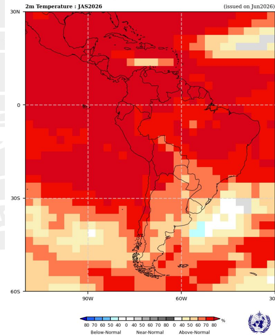
Probabilistic Multi-Model Ensemble Forecast CPTEC, ECMWF, Melbourne, Montreal, Offenbach, Seoul, Washington
